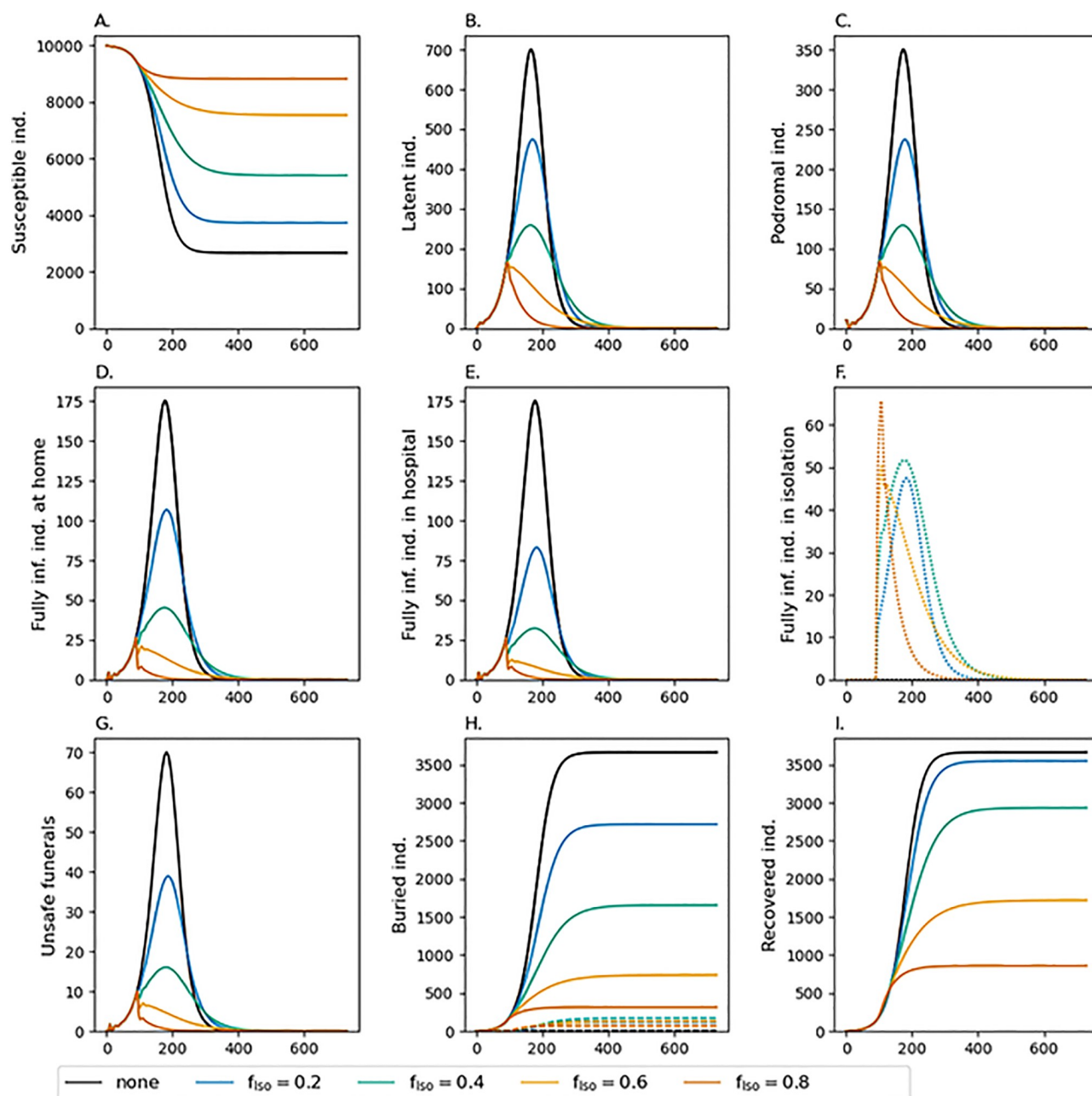
Fig 2. Fraction of isolated f_{iso} infections. Shown are the dynamics of the model for different choices of f_{iso} (colors). Different panels show the number of susceptibles, infected in various phases, unsafe funerals, buried individuals, and recoveries. In the different phases of the infections, the numbers are accumulated over the respective Erlang stages. Isolated infections are shown as dotted lines. In panel (H) the dashed lines show those who have received a safe funeral. Isolation starts at time t_{iso} = 90 days. Moderate mortality is assumed (see S7 Table). All other model parameters used for the simulations are listed in Tables S1–S6 Tables.
