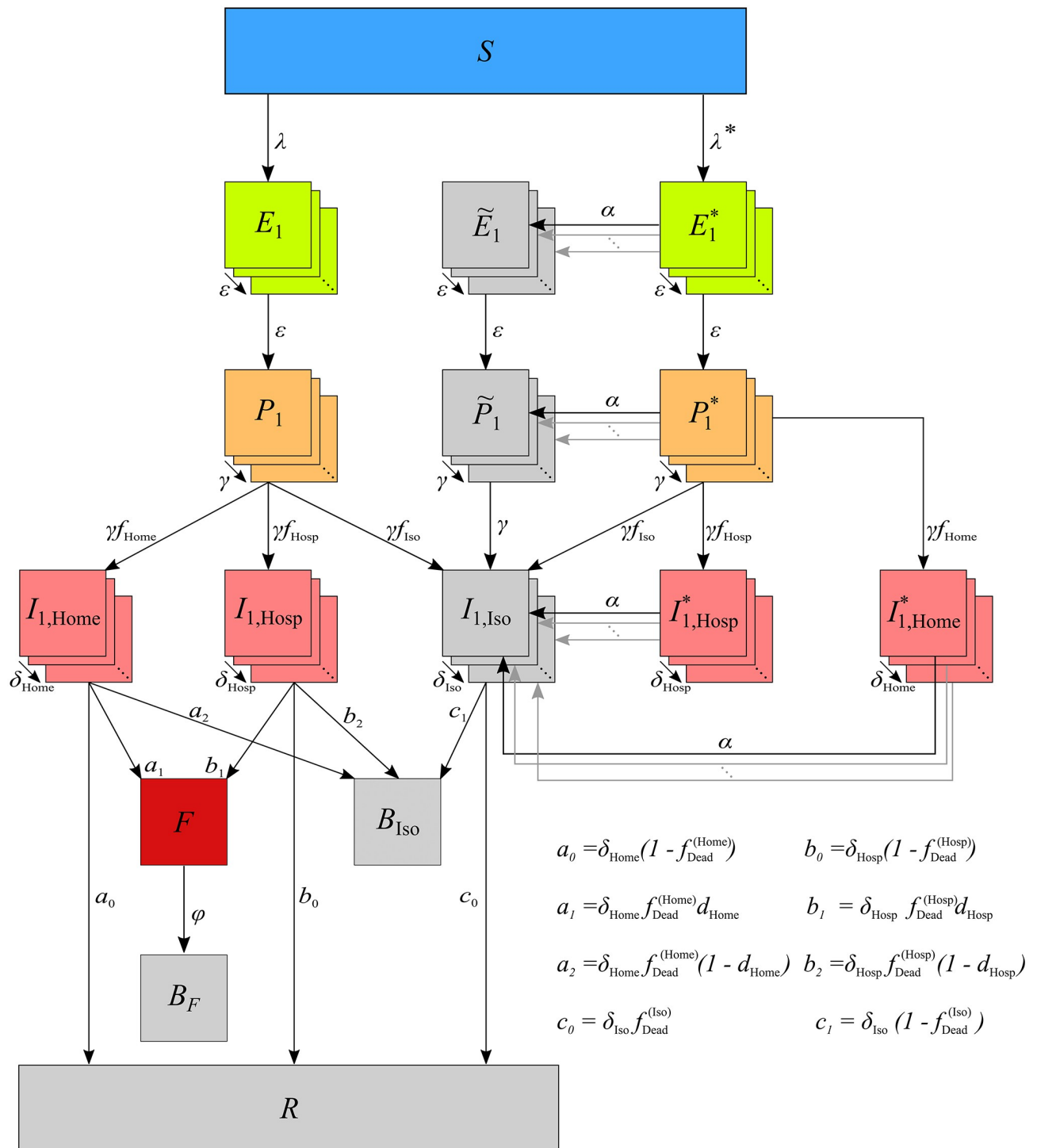
Fig 1. Model. Stages are depicted as boxes, arrows show transition rates. The entire population is grouped into the susceptibles ( S ), the infected which are further classified into the latent ( E ), the prodromal ( P ), the fully infectious at home, ( I_{\text{Home}} ), in hospital, ( I_{\text{Hosp}} ), and in isolation, ( I_{\text{Iso}} ), and the recovered ( R ). The dead are classified into those awaiting an unsafe Funeral ( F )—still infectious, after funeral ( B_F ), or buried safely ( B_{\text{Iso}} ). Trace back is modeled through the force of infection for infections subject to trace back \lambda^* , resulting in individuals in transient stage ( E^* , P^* , I_{\text{Home}}^* , I_{\text{Hosp}}^* ) who will get traced back later, and those ( \tilde{E} , \tilde{P} , I_{\text{Iso}} ) who have already been traced back or diagnosed—these are isolated; \lambda and E , P , I_{\text{Home}} , I_{\text{Hosp}} describe infections not subject to trace back. The rates \varepsilon , \gamma , \delta_{\text{Home}} , \delta_{\text{Hosp}} , \delta_{\text{Iso}} describe the progression of the infections. \alpha is the rate of successful trace back, \varphi the one of funerals, d_{\text{Home}} , d_{\text{Hosp}} indicate the fractions of safe funerals of non-diagnosed individuals. f_{\text{Home}} , f_{\text{Hosp}} , f_{\text{Iso}} are the fractions of fully infectious in different treatment, where f_{\text{Dead}}^{(\text{Home})} , f_{\text{Dead}}^{(\text{Hosp})} , f_{\text{Dead}}^{(\text{Iso})} are the related death rates.
