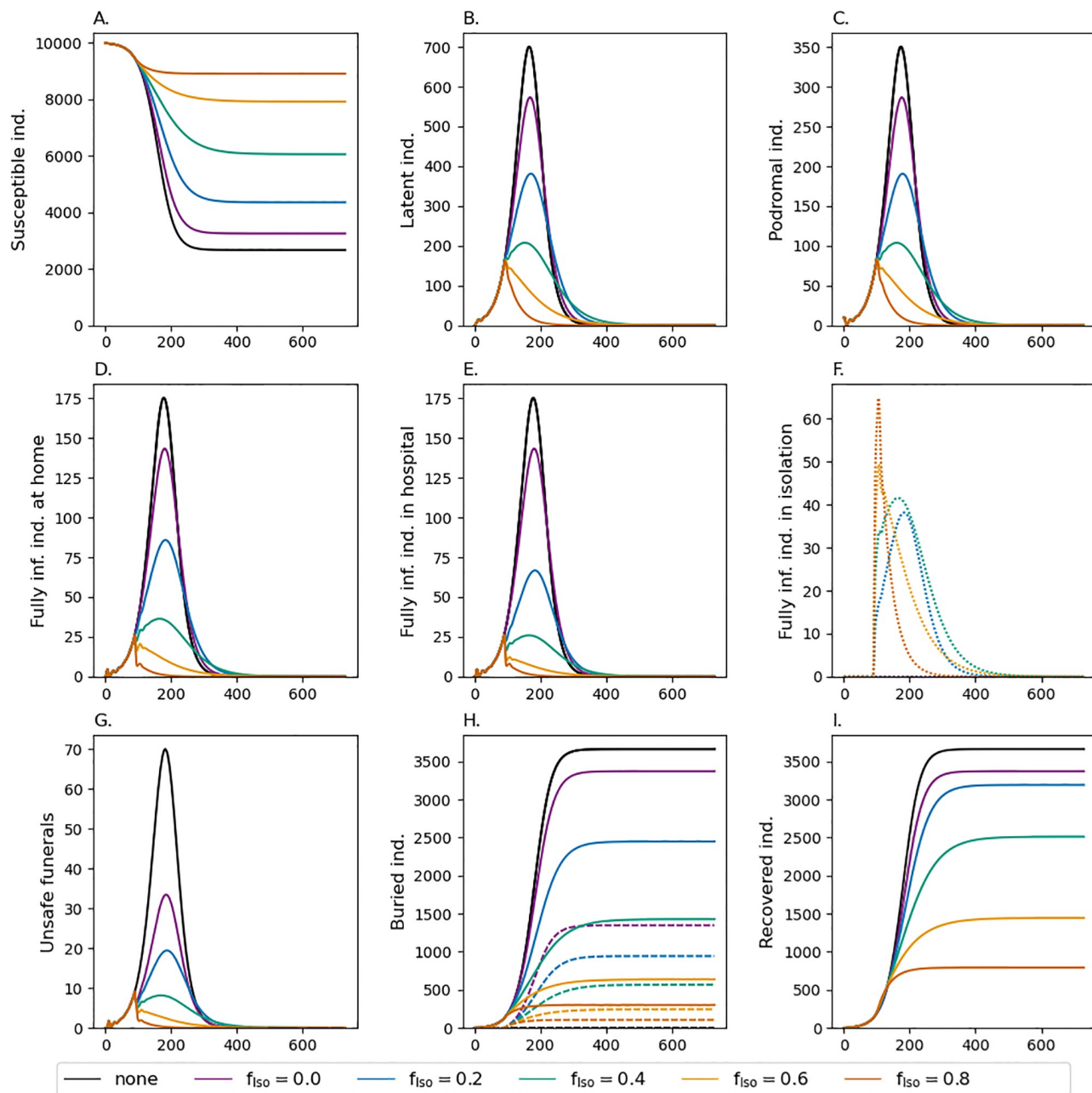
Fig 3. Safe funeral practices. See Fig 2 but combined with safe funeral practices. The fraction of safe funerals after death at home and in hospital are assumed to be d_{\text{Home}} = 0.16 and d_{\text{Hosp}} = 0.8 , respectively.
