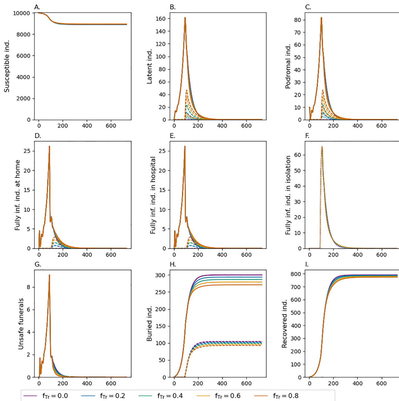
Fig 4. Extent of back-tracking. Effect of fraction of infected individuals who will be traced back f_{Tr} , when the fraction of infections that are isolated is f_{iso} = 0.8 with additional safe funeral practices for lethal cases that occurred outside isolation ( d_{Home} = 0.16 and d_{Hosp} = 0.8 ). In panels (B-F) the dashed lines show the number of infections that will be traced back at some time in the future (not yet isolated) or are currently traced back (and in isolation). The dotted lines show all individuals currently in isolation. In panel (H) the dashed lines show the numbers of safe funerals that were conducted.
