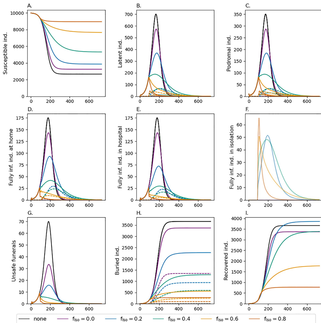
Fig 5. Combination of interventions. See S3 Fig but with additional safe funeral practices for lethal cases that occurred outside isolation ( d_{Home} = 0.16 and d_{Hosp} = 0.8 ). The average trace-back time is D_T = 21 days. A fraction f_{Tr} = 0.8 of contacts of infections in isolation are subject to back-tracking.
